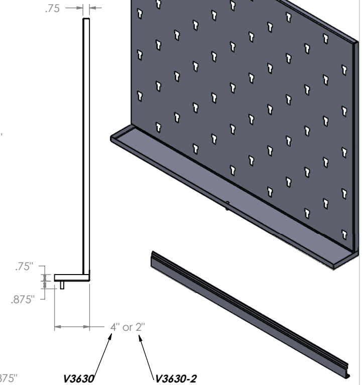
Wall Mount Bracket
